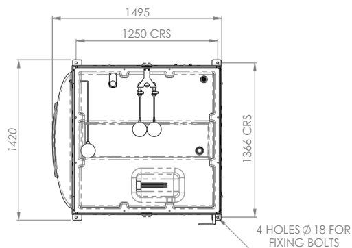
PLAN VIEWS WITH TANK LID OMITTED
